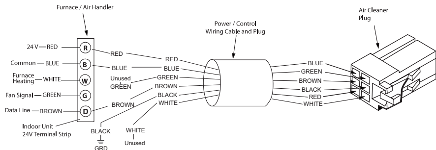
Figure 20 - Wiring Diagram Communicating Mode
