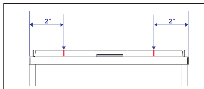
Figure 17 Duct Flanges
