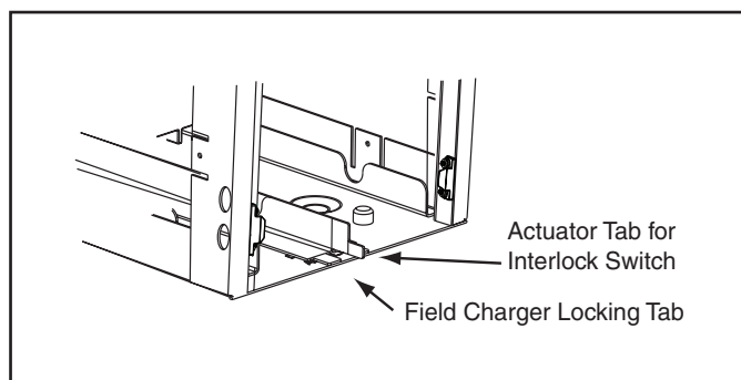
Figure 16 Locking Tab
