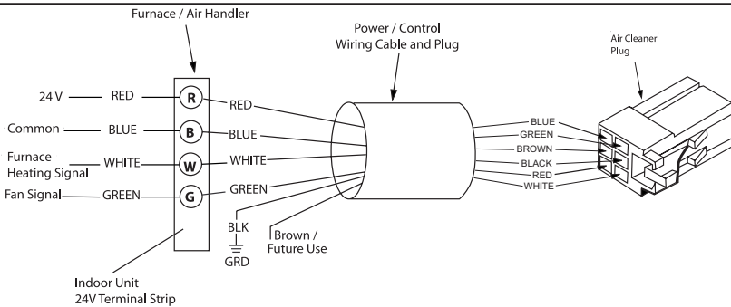
Figure 20A - Wiring Diagram for 24 V Mode
