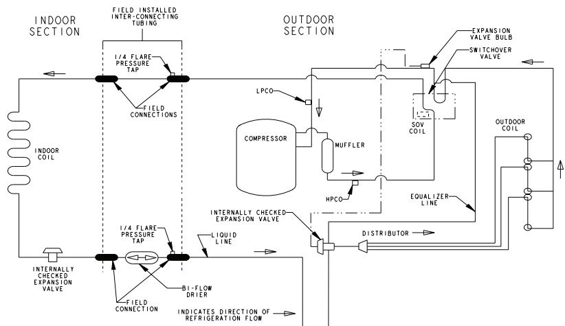
Heating Refrigeration Cycle
