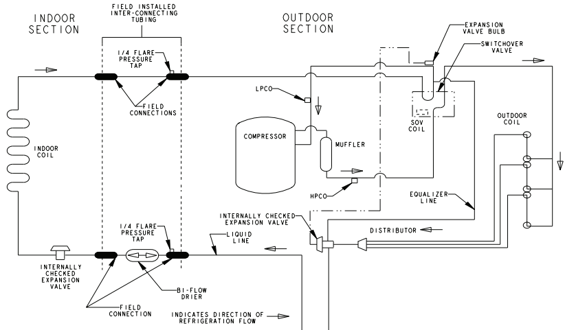
Cooling Refrigeration Cycle
