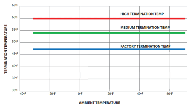
DEFROST TERMINATION PROFILES
